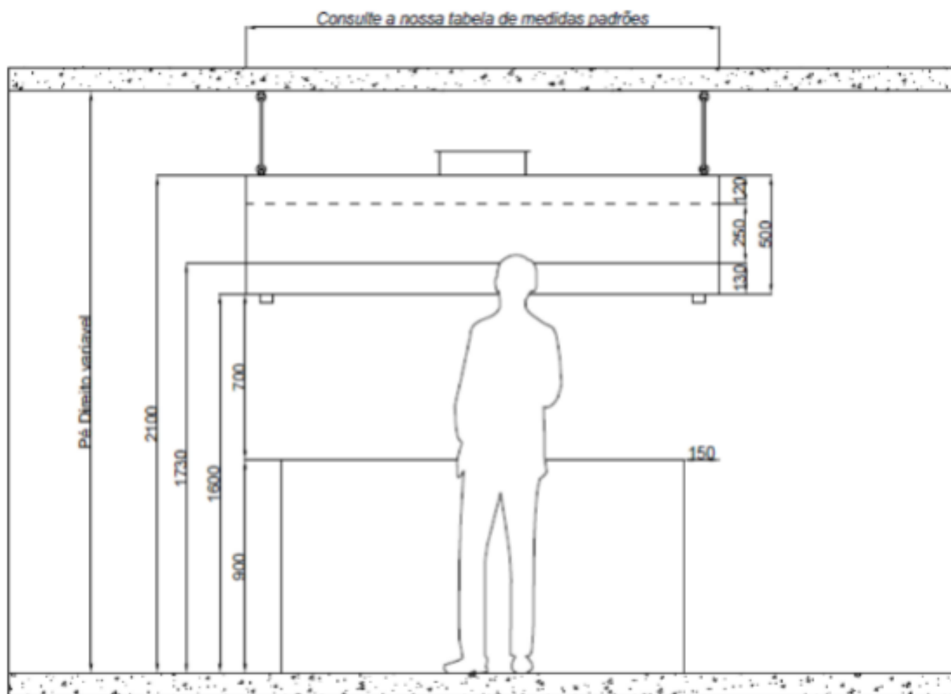
Vista Frontal
